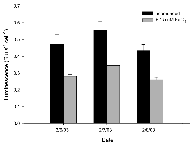
Figure 5. Influence of added FeCl 3 on perceived Fe bioavailability. Luminescence measures from bioreporter cells grown in 0.2- \mu m filtered surface water and Fe (1.5 nM) amended 0.2- \mu m filtered surface water from the center of the FeCycle patch for 6 through 8 February. Although Fe concentrations and Fe bioavailability peaked during this period, the results indicate that high-affinity transporters could still be further suppressed by added Fe, and as such the Fe availability was still in part constraining the community.
