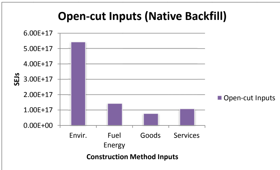
Figure 10. EVE EMERGY inputs for alternative B (Open-cut).
